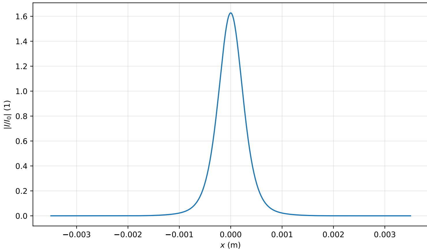
Intensity profile I(x, y = 0, z = 1.911m)/I_0 , P_{in}=0.9P_{cr} , artificial time
